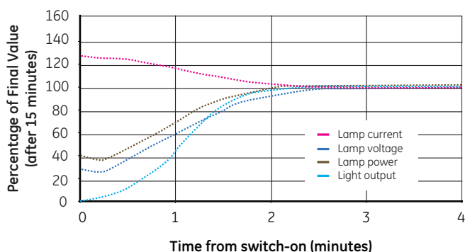
Typical Warm-up CMH 20W SuperMini
