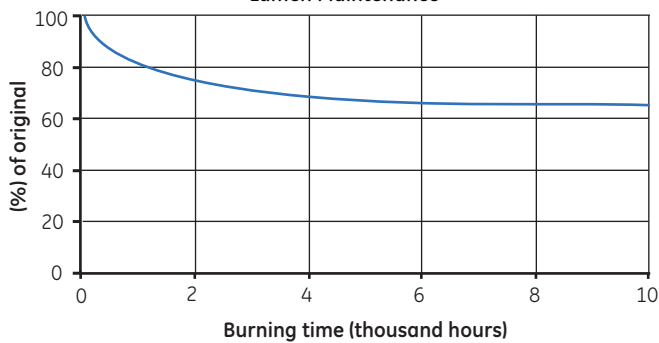
CMH35W SuperMini 930 Lumen Maintenance
