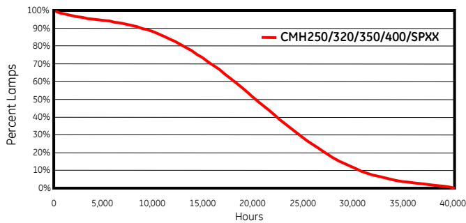
High Watt CMH® Lamp Mortality
