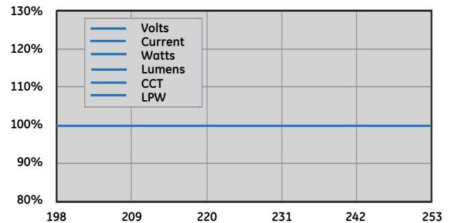
CMH Lamp performance as a function of supply voltage on an electronic ballast
