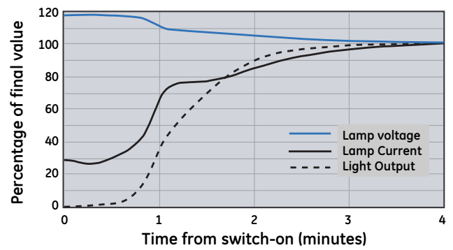
CMH Lamp performance as a function of supply voltage on a 220V Reference Ballast
