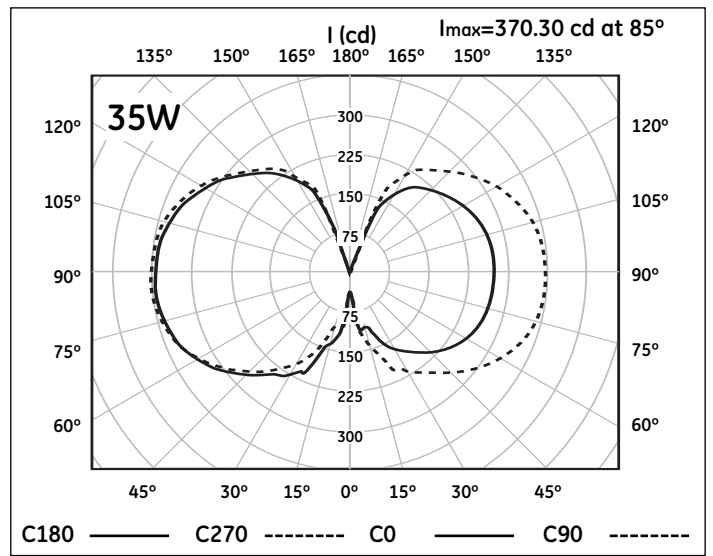
Horizontal plane polar intensity curve
