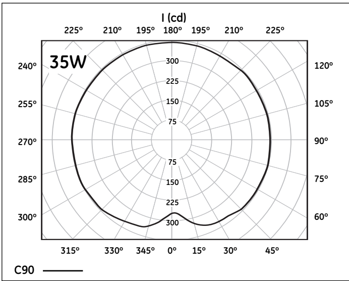
Vertical plane polar intensity curve
