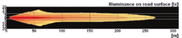
STANDARD 5" x 7" HALOGEN HIGH BEAM
