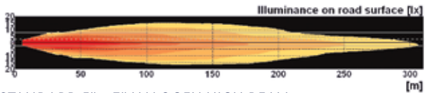
STANDARD 5" x 7" HALOGEN HIGH BEAM
